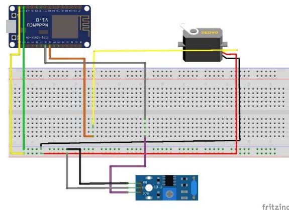
Gambar 3. Rangkaian Hardware
